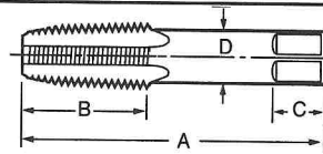
General Dimensions
