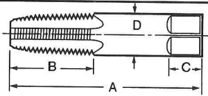
General Dimensions
